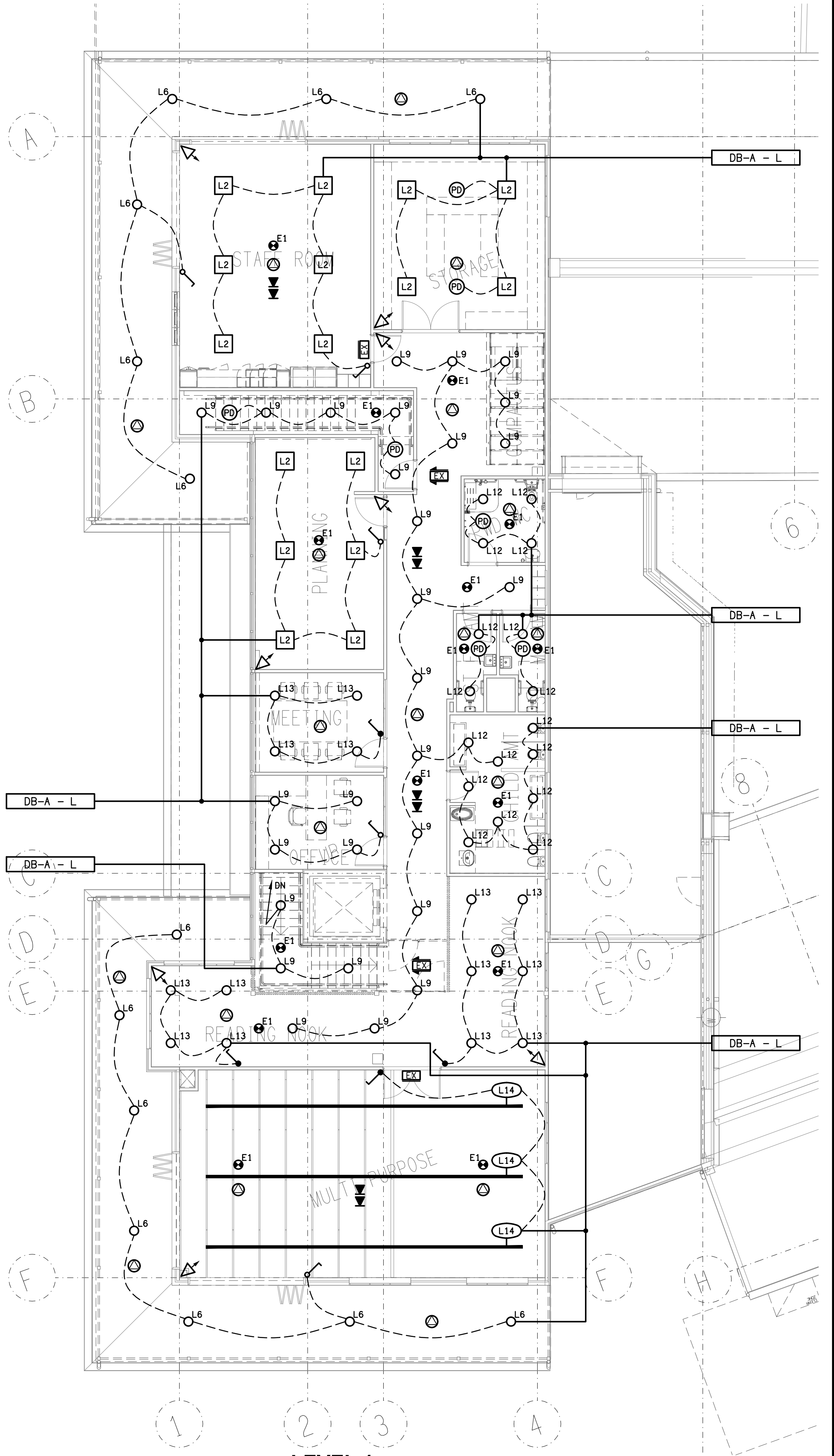
LEVEL 1 REFLECTED CEILING PLAN SCALE 1: 100
